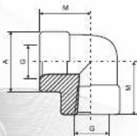
90° Kolana FF-NPT 3000 LBS
